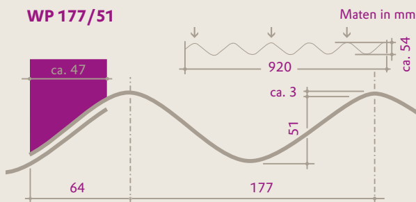
Diameter PLEXIGLAS® Resist WP 177/51 (maten in mm)
