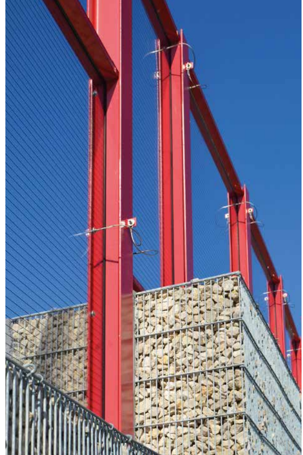
Noise barrier, Pirmasens PLEXIGLAS® Soundstop GS CC, 15 mm
