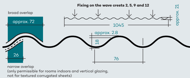
Cross-section of PLEXIGLAS® Resist WP 76/18/2.8
