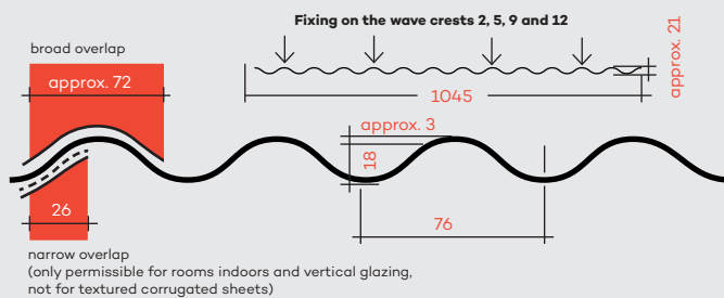
Cross-section of PLEXIGLAS® Resist WP 76/18/3
