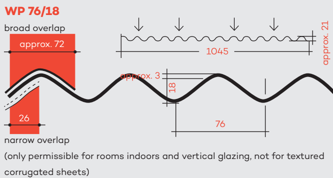
Cross-section of PLEXIGLAS® Resist WP 76/18 (dimensions in mm)
