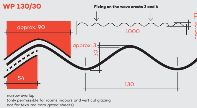
Cross-section of PLEXIGLAS® Resist WP 130/30 (dimensions in mm)
