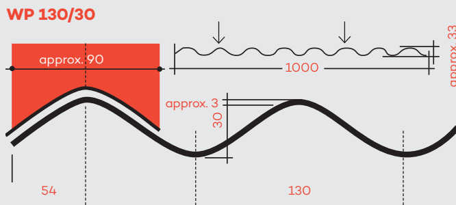
Cross-section of PLEXIGLAS® Resist WP 130/30 (dimensions in mm)
