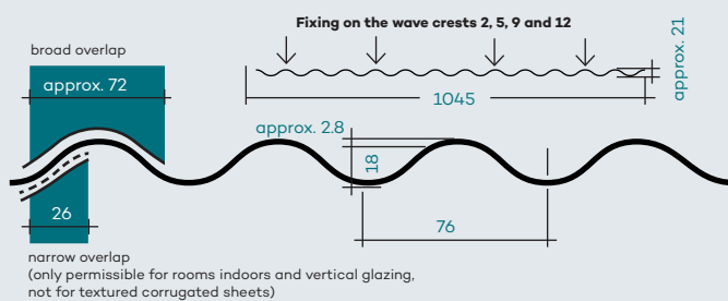
Cross-section of PLEXIGLAS® Heatstop Cool Blue WP 76/18/2.8
