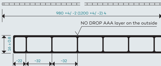
Section of PLEXIGLAS® Resist AAA SDP 16/980 (Dimensions in mm)
