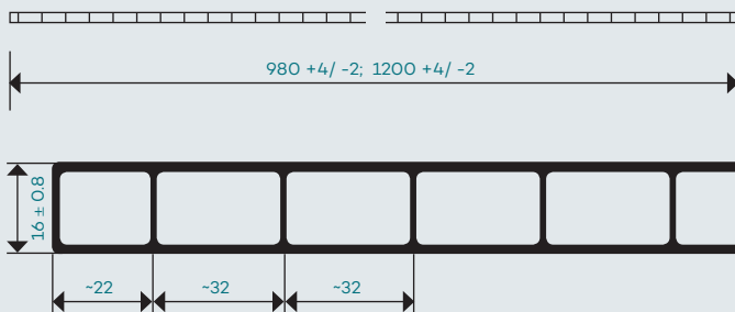
Section of PLEXIGLAS® Heatstop Cool Blue SDP 16/ (Dimension in mm)
