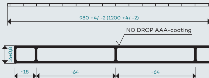
Dwarsdoorsnede PLEXIGLAS® Resist AAA SDP 16-64 (afmetingen in mm)
