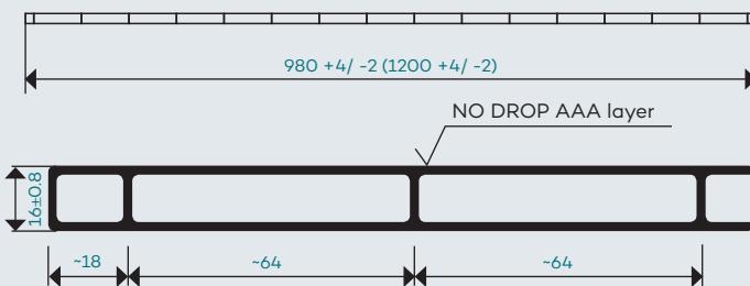
Section of PLEXIGLAS® Heatstop Cool Blue AAA SDP 16-64 (Dimensions in mm)
